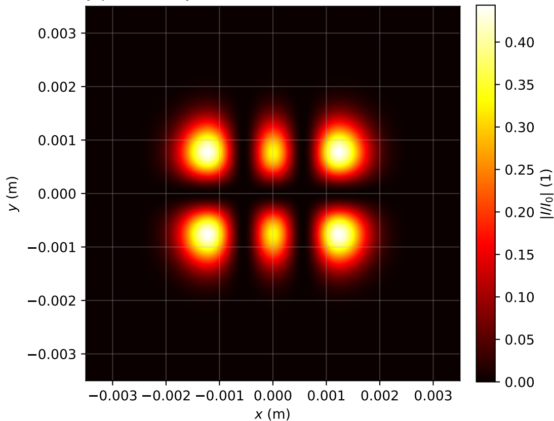
Intensity profile I(x, y, z = 2.388)/I_0 , P_{in}=0.5P_{cr} , artificial time
